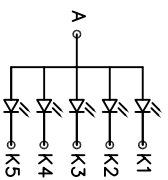
B/L CIRCUIT DIAGRAM LED:IF = 100mA,VF=3.2V
